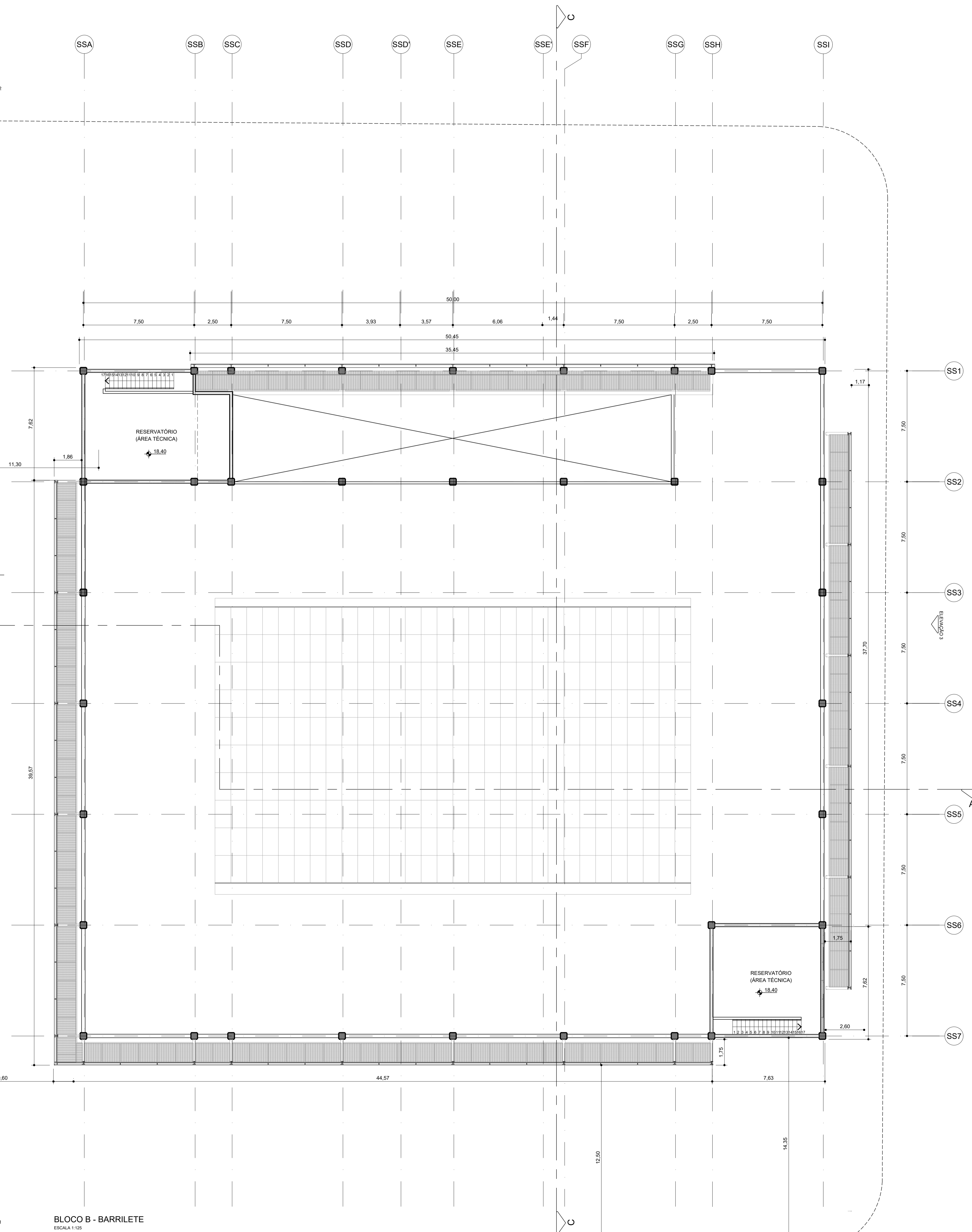
BLOCO B - BARRILETE ESCALA 1:125
